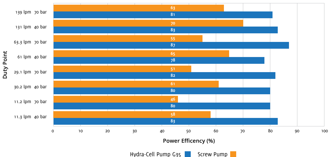
Pump-Shaft to hydraulic power efficiency
